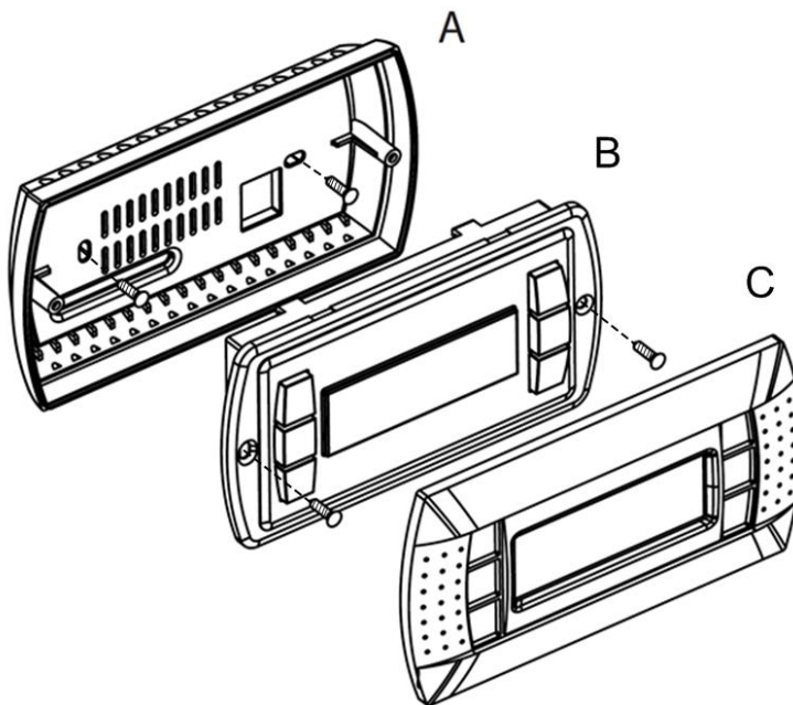
Figure 23 - Montage mural
